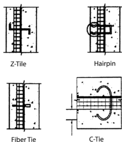
Figure 42 Tension/compression ties.
