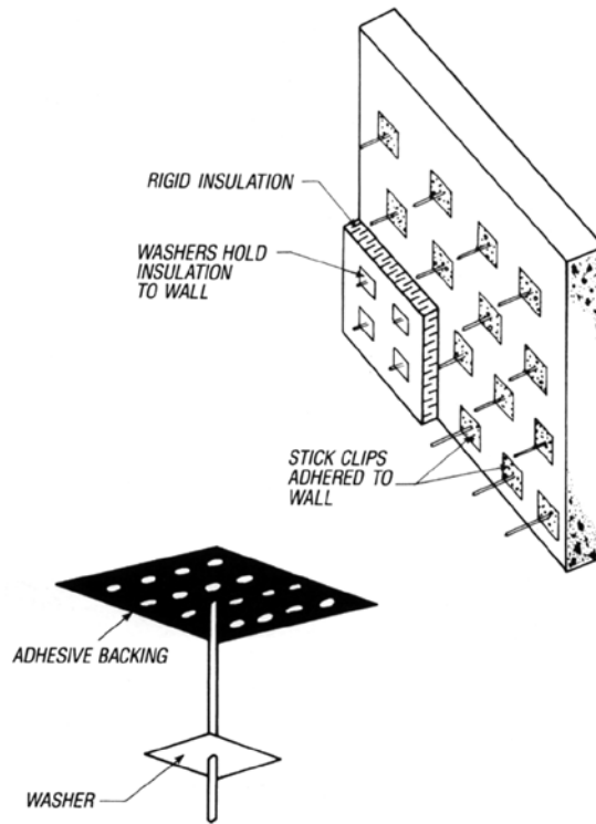
Figure 33 Use of stick clips to install rigid insulation.
