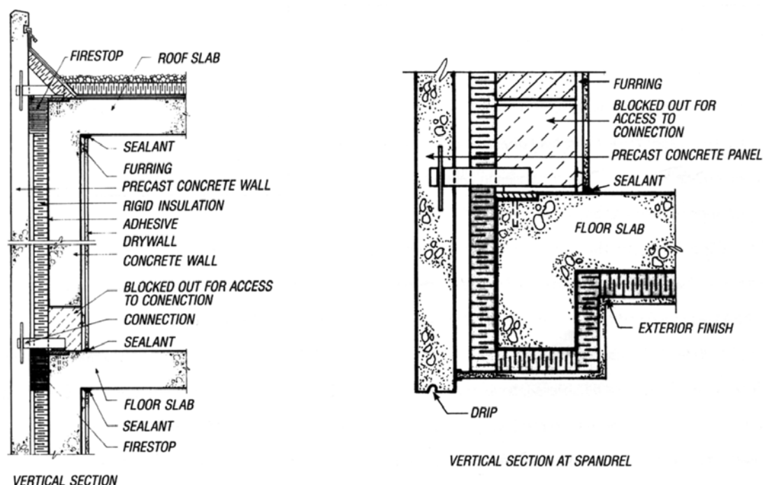
Figure 35 Cladding erected over previously erected wall.
