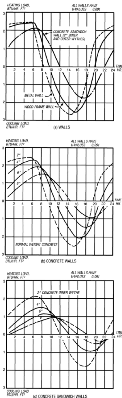
Figure 16 a-c Heating and cooling load comparisons.
