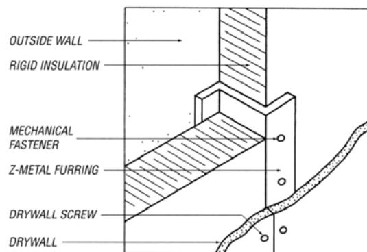
Figure 34 Furring systems.
