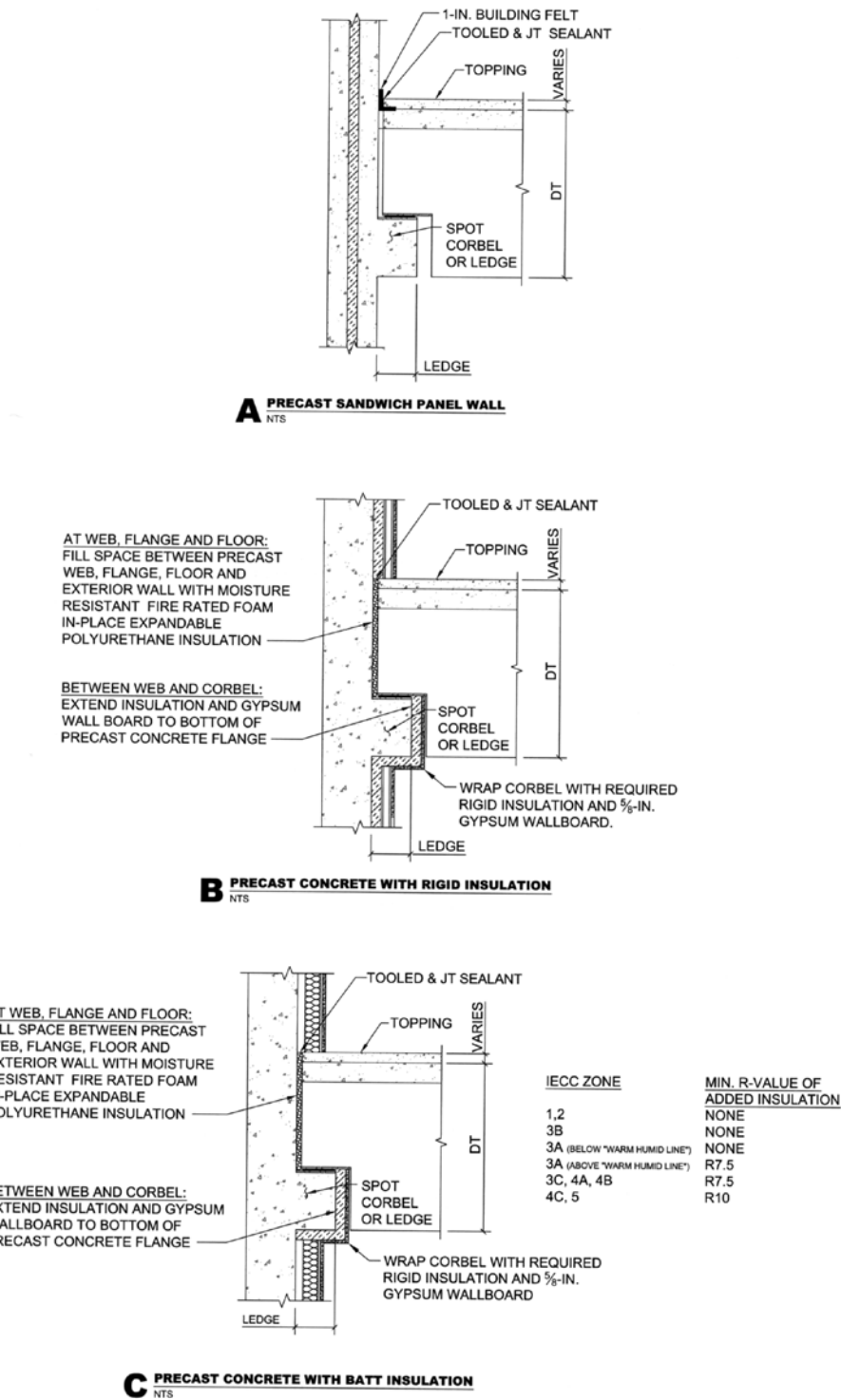
Figure 28 Typical loadbearing spandrel with corbel/dapped DT detail.
