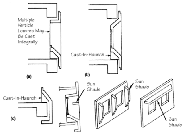
Figure 1 Shading elements.
